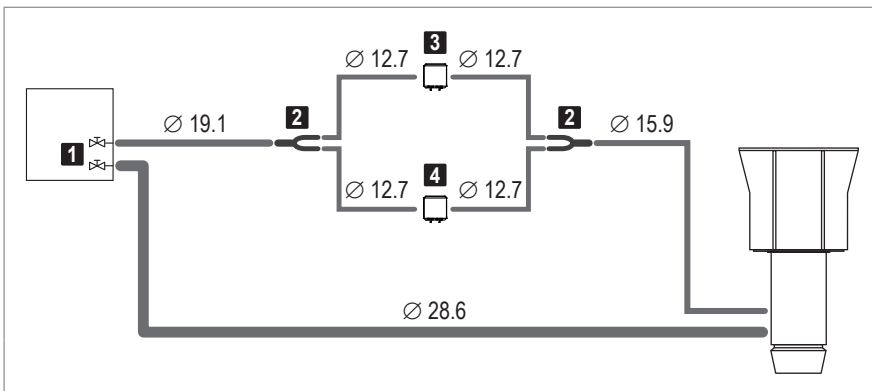
Fig. D14: Refrigerant pipes for Belaria® VRF (67) (pipe diameter in mm)
