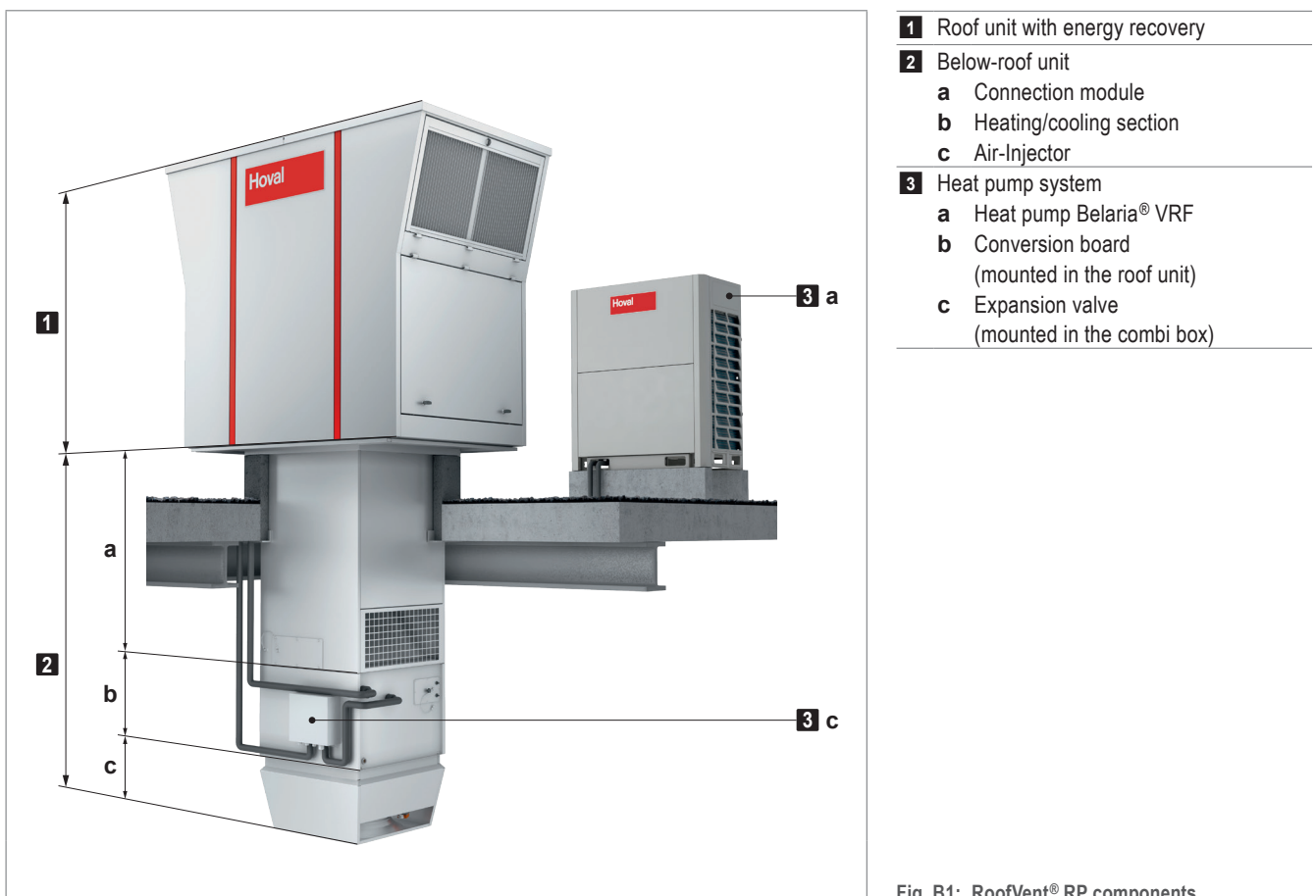
Fig. B1: RoofVent® RP components
