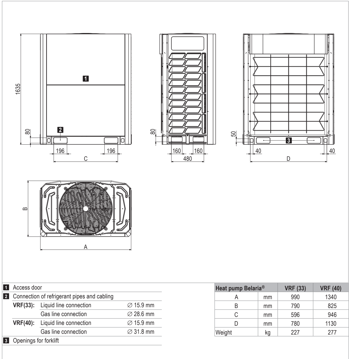
Fig. B6: Dimensions and weights Belaria® VRF (33, 40)
