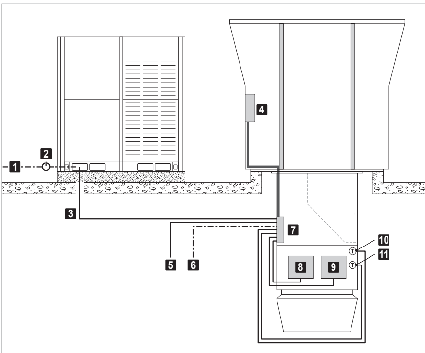
Fig. D18: Electrical connection of the heat pump system for RoofVent® RP-9
