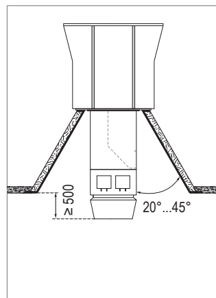
Fig. D8: Roof frame with conical side walls
