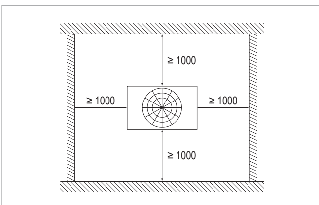
Fig. D3: Minimum distances for the heat pump (dimensions in mm)
