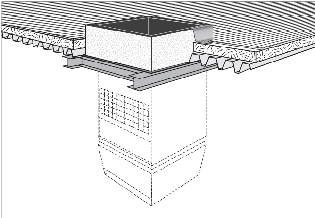
Fig. D6: Conceptual drawing of the roof frame
