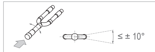
Fig. D10: Installation of the branching kit
