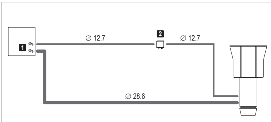
Fig. D13: Refrigerant pipes for Belaria® VRF (40) (pipe diameter in mm)
