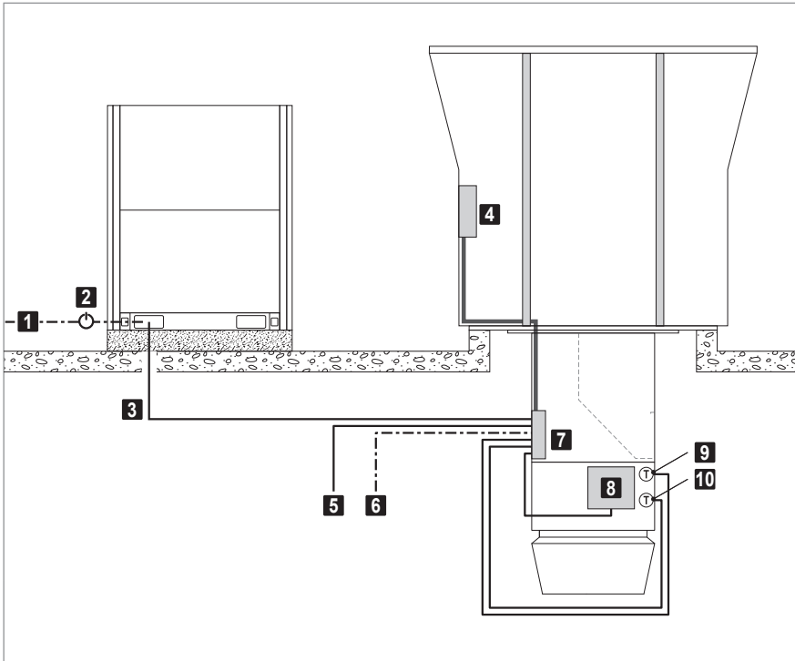
Fig. D17: Electrical connection of the heat pump system for RoofVent® RP-6
