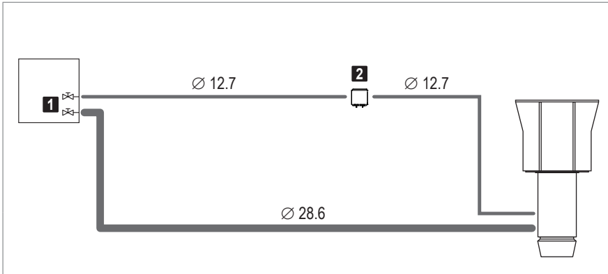
Fig. D12: Refrigerant pipes for Belaria® VRF (33) (pipe diameter in mm)
