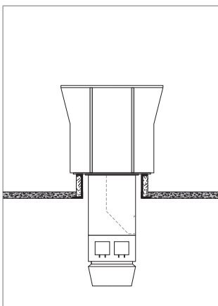
Fig. D7: Roof frame with straight side walls
