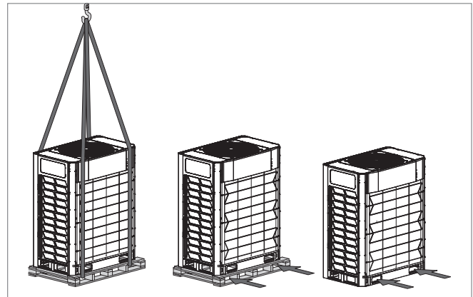
Fig. D1: Lifting the heat pump
