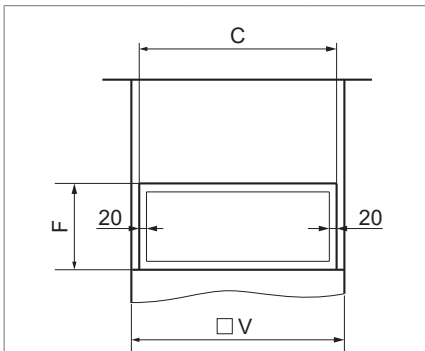
Fig. D9: Extract air duct
