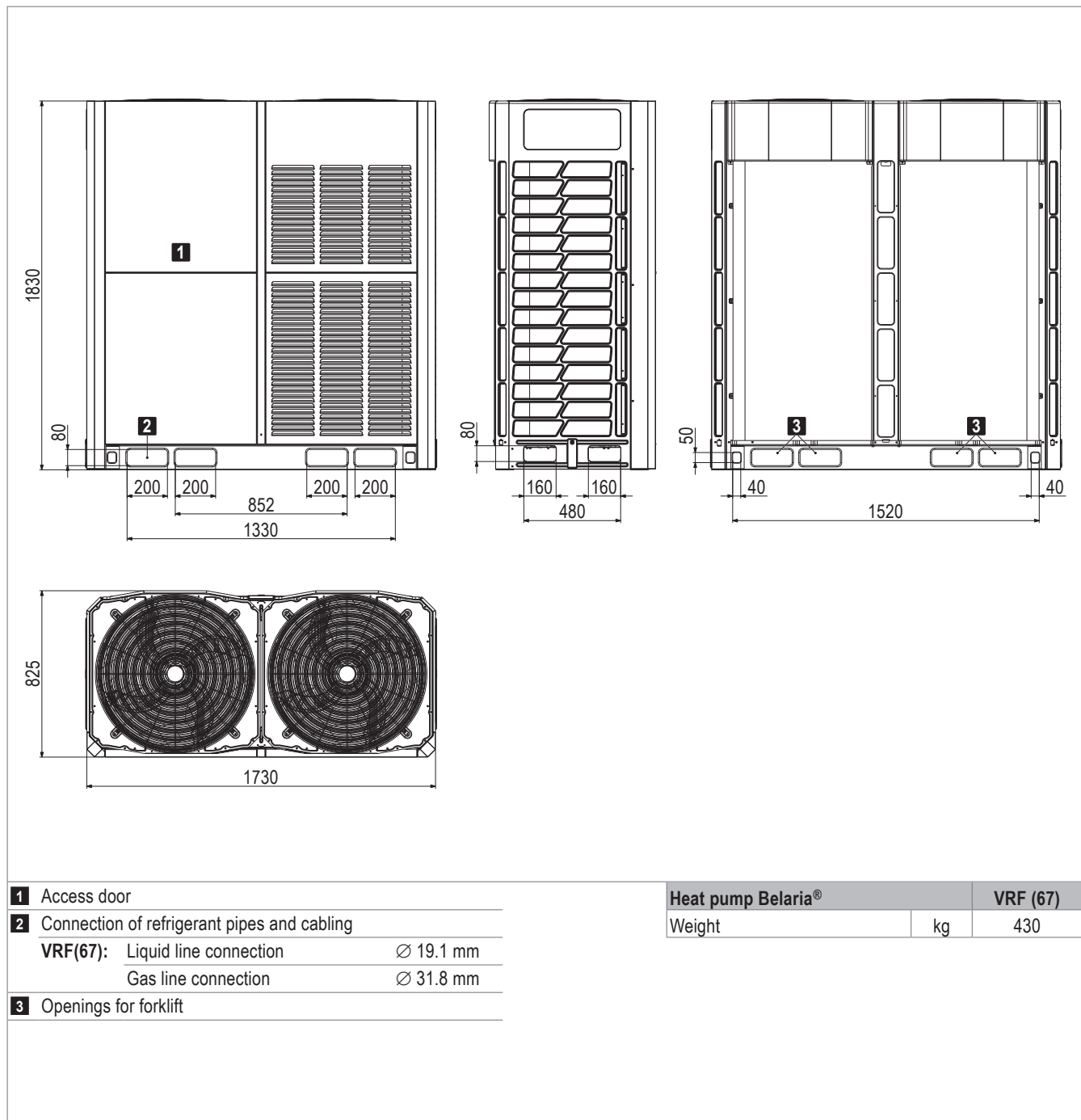
Fig. B7: Dimensions and weights Belaria® VRF (67)
