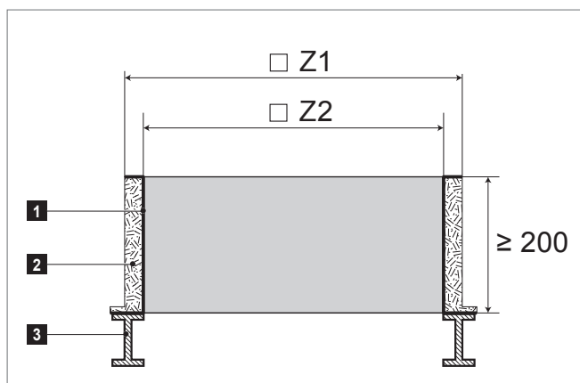
Fig. D5: Installation of RoofVent® units in the roof frame (dimensions in mm)
